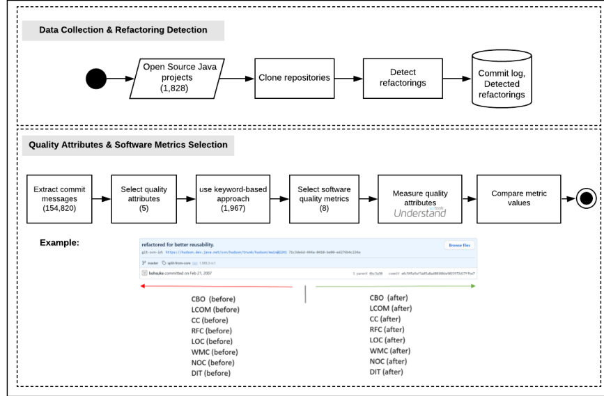
Fig. 1: Empirical study design overview.
